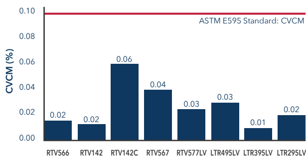
ASTM E595 Results: CVCM (≤0.10%)
